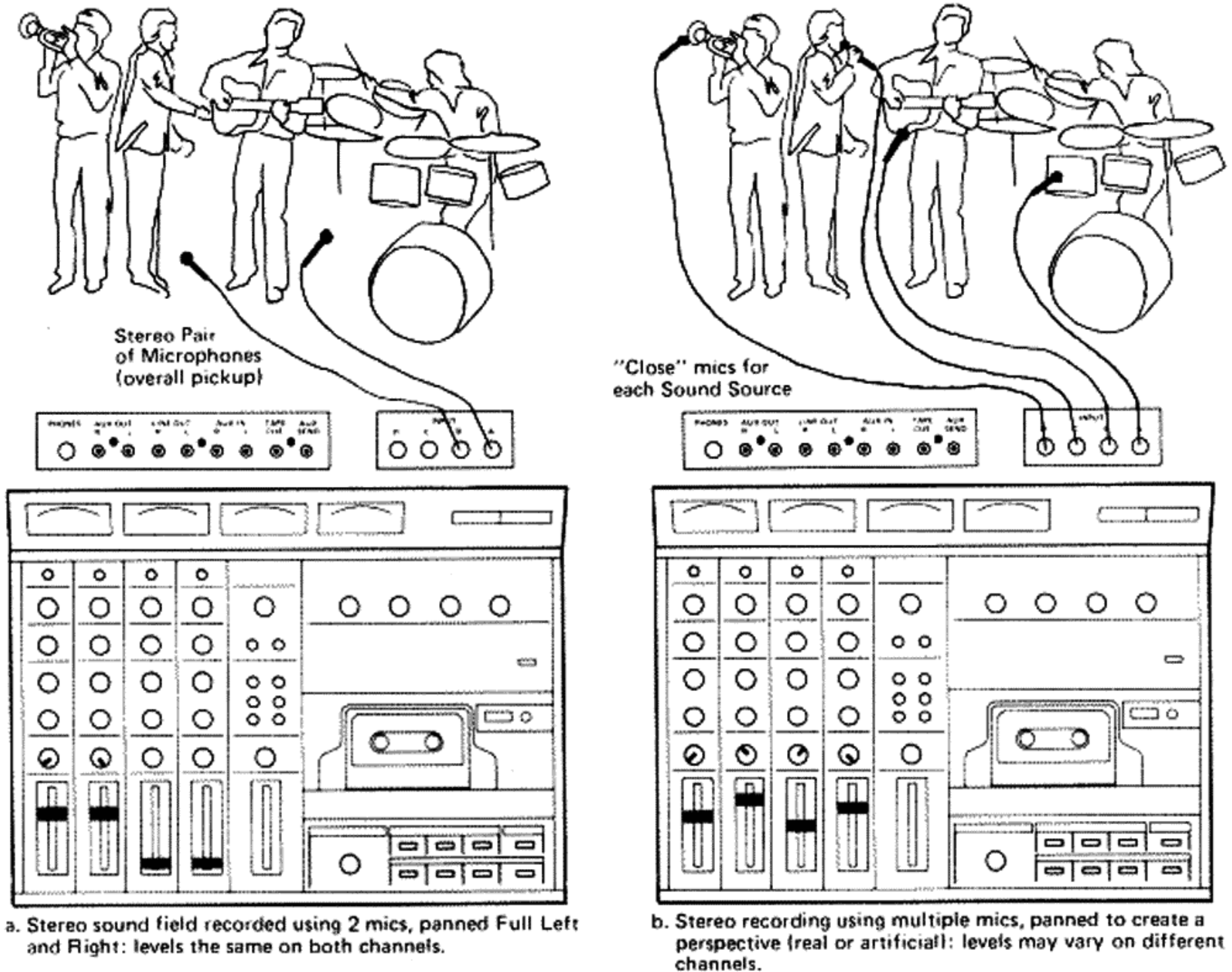
Figure 14 - Pictorial Representation of Stereo Recording
