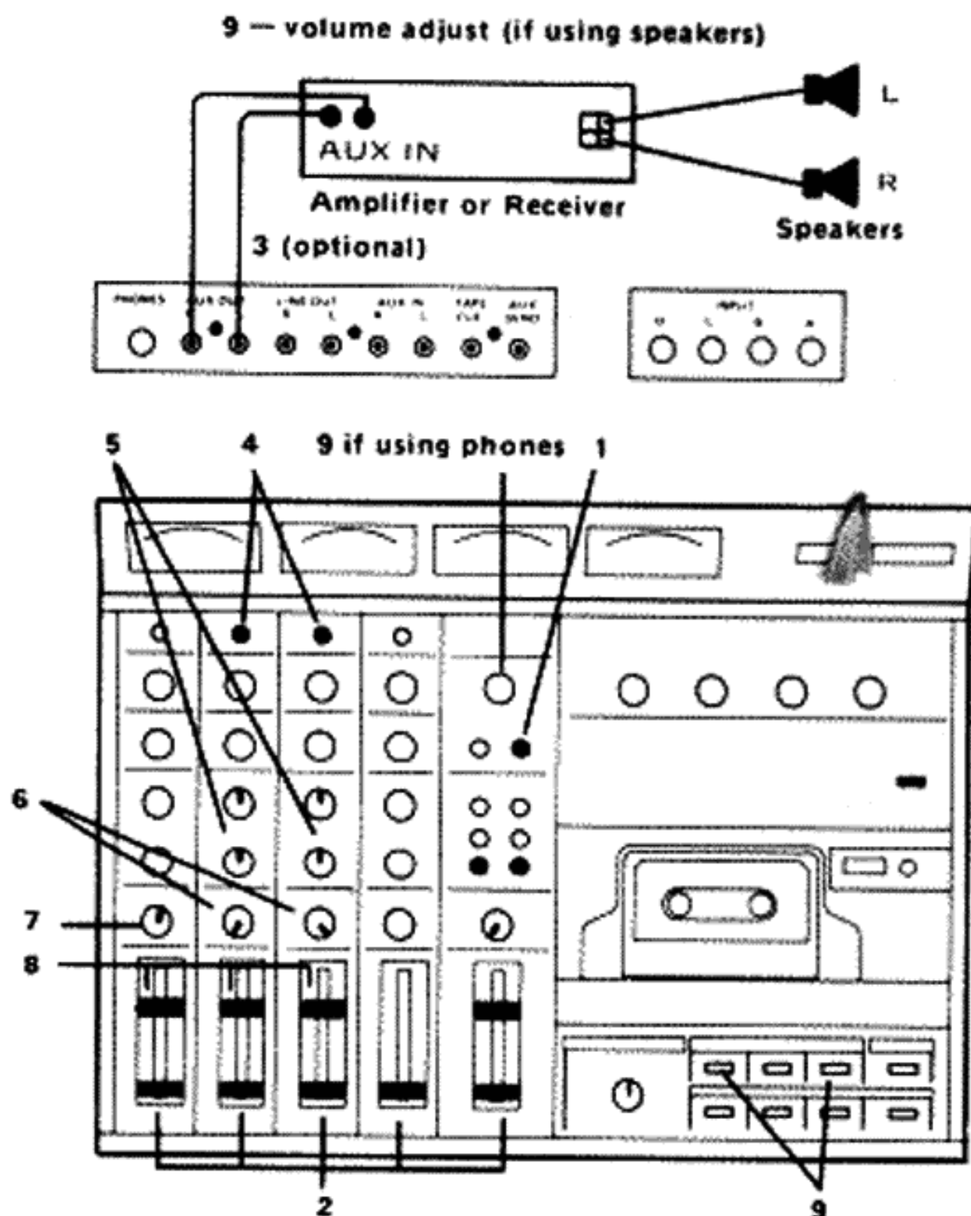
Figure 16 - Typical Setup for Stereo Playback to Evaluate Cassette
