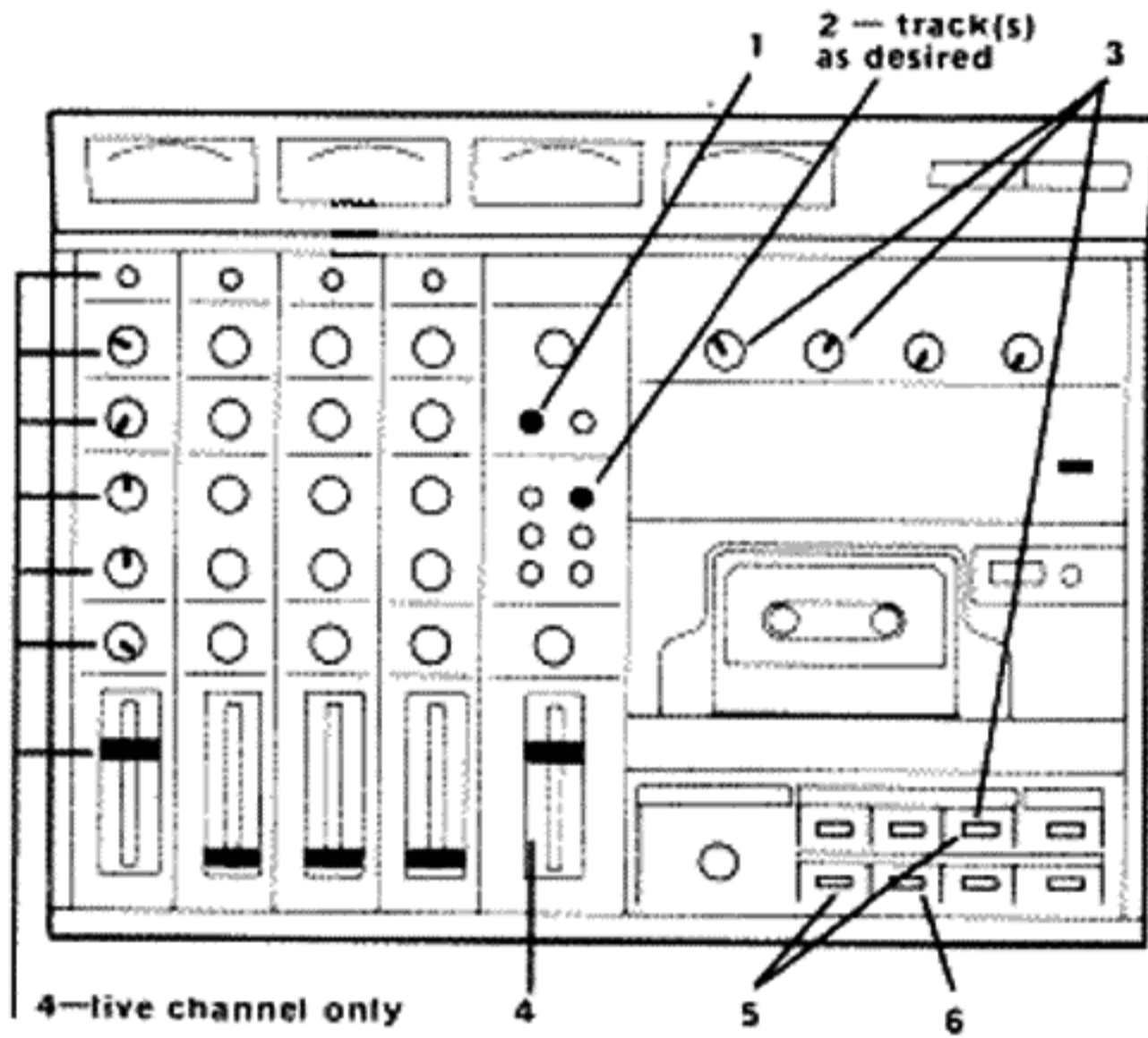
Figure 21 - Typical Setup for Punch-In Recording
